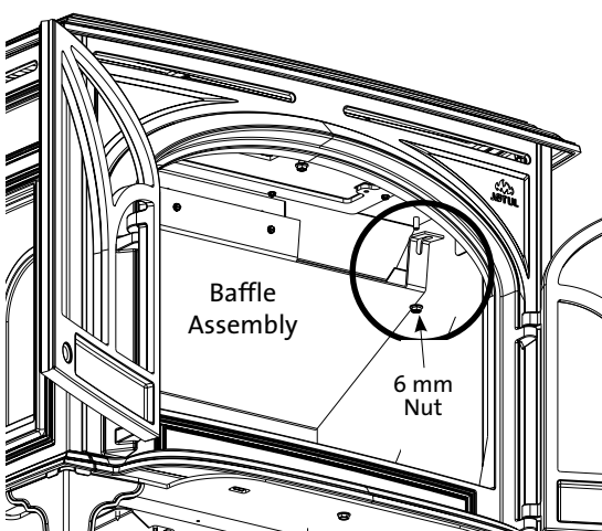
Figure 31. Baffle Assembly location. Remove two 6 mm nuts to detach it from the firebox.
