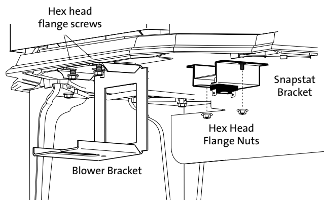
Figure 42. Attach Snapstat and Blower Brackets.
