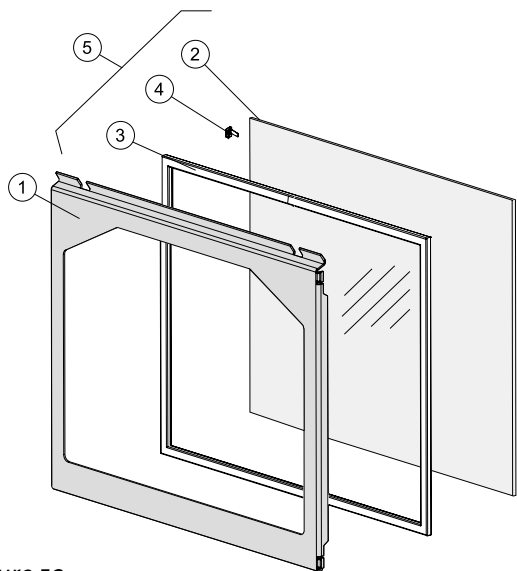
Figure 59. GF 500 DV Glass Assembly
