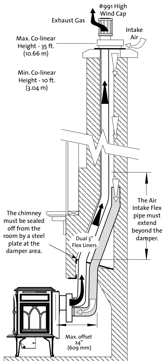
Figure 18. Co-linear Adaptor installed through a masonry chimney. M&G DuraVent components shown.
