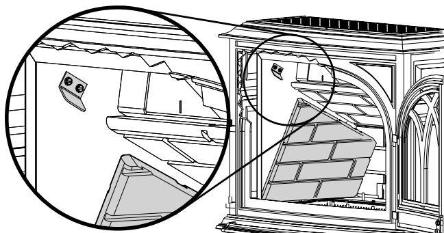
Figure 40. Install the Brick Panels.
