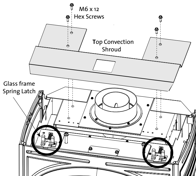
Figure 2a. Remove the Top Convection Shroud and disengage the glass frame latches.
