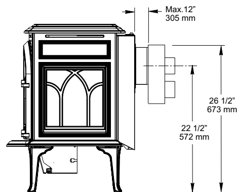
Figure 17. M&G DuraVent #923GCL Co-linear Adaptor.
