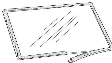
Figure 55. Wrap the gasket around the glass panel.
