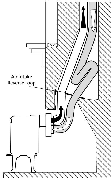
Figure 16. A “reverse loop” in the air intake run can help maintain draft strength.
