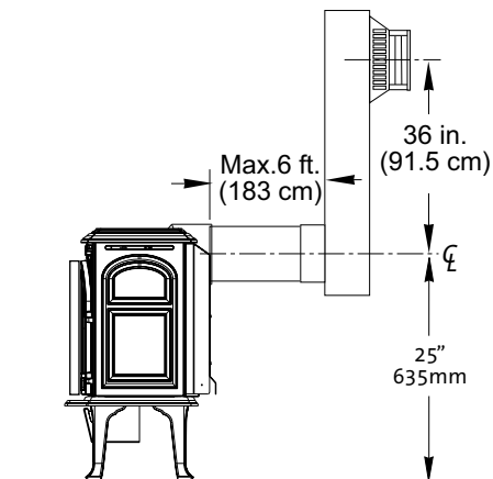
Figure 18. Maximum Horizontal with 36" Snorkel Termination. Remove Baffle Wing 226873 for all Snorkel terminations.
