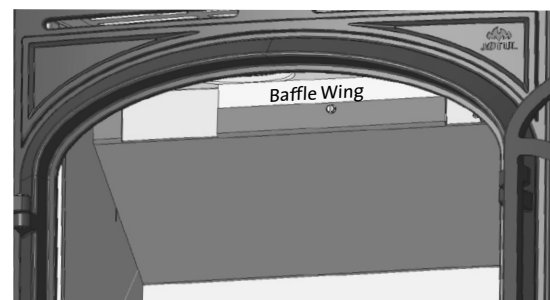
Figure 25a. For PROPANE, remove the Baffle Wing from the Exhaust Baffle.
